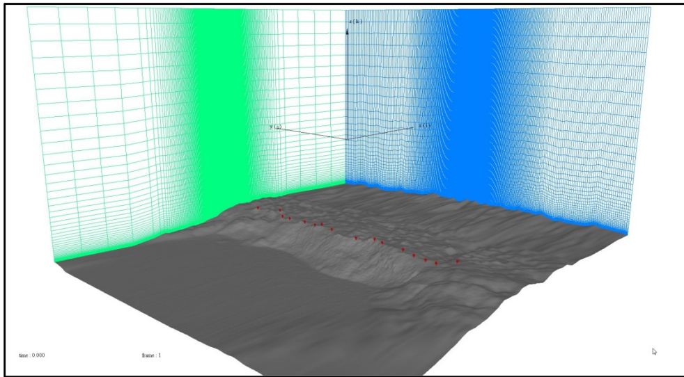
Fig.2 - LES CFD domain and calculation mesh constructed by RIAM-COMPACT®
