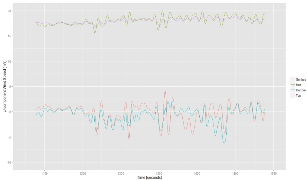
Fig.4 - Time Series of U component wind speed at rotor top, hub, rotor bottom and ground surface level at turbine T12
