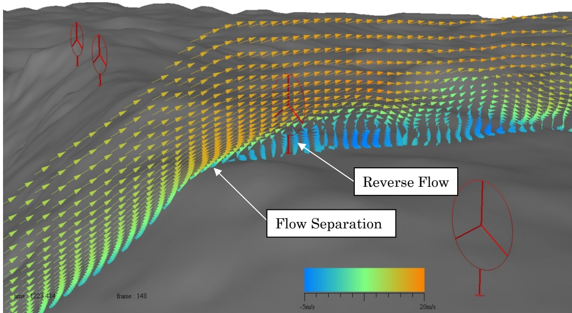
Fig.3 - Instantaneous vector plot at turbine T12
