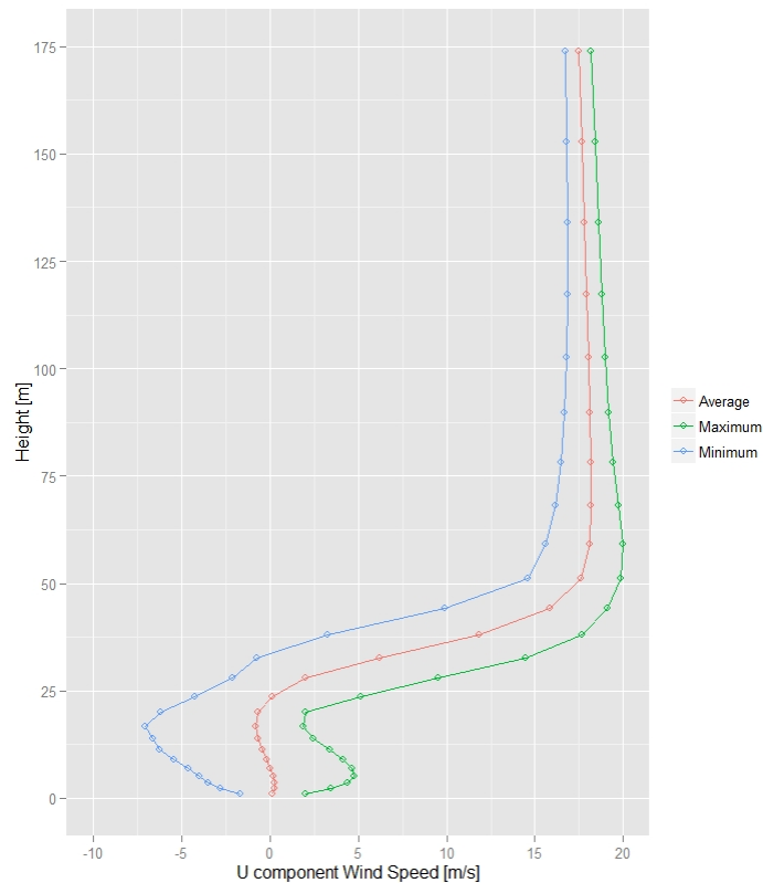
Fig.5 - Vertical Shear Profile predicted by RIAM-COMAPCT®
