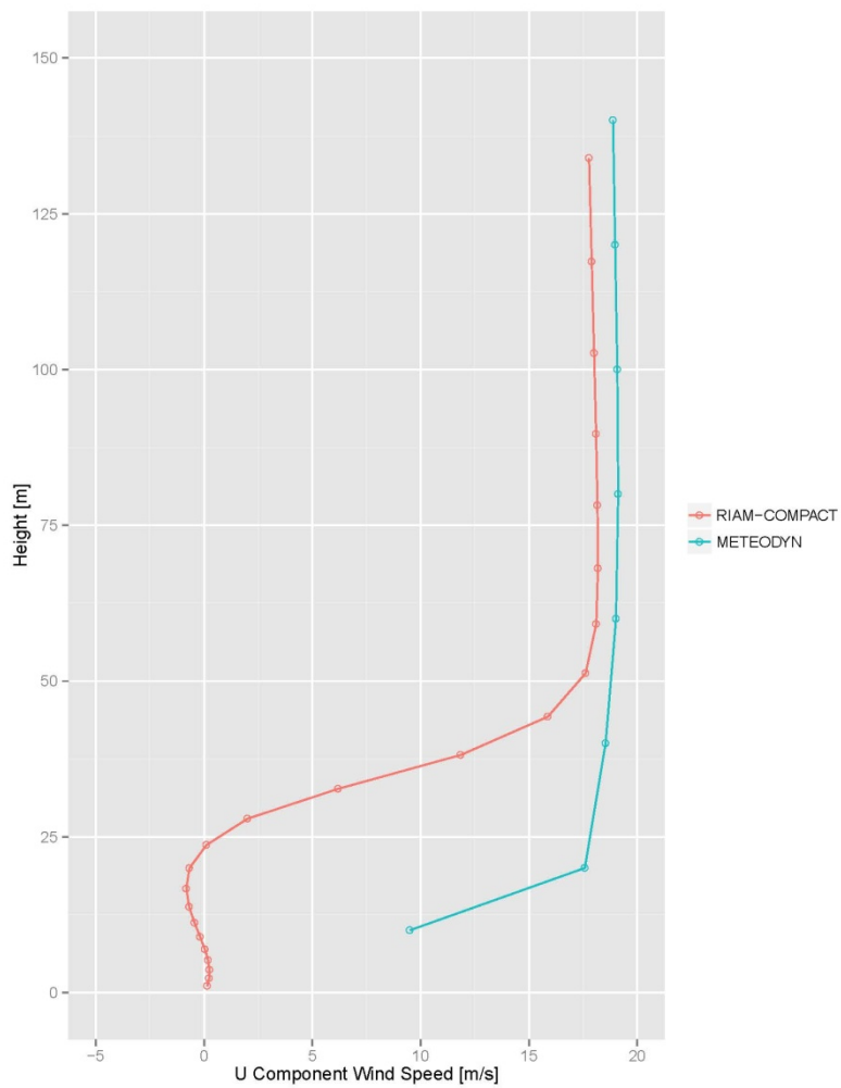
Fig.6 - Comparison of vertical shear profile between the wind flows simulated by RIAM-COMPACT® and METEODYN
