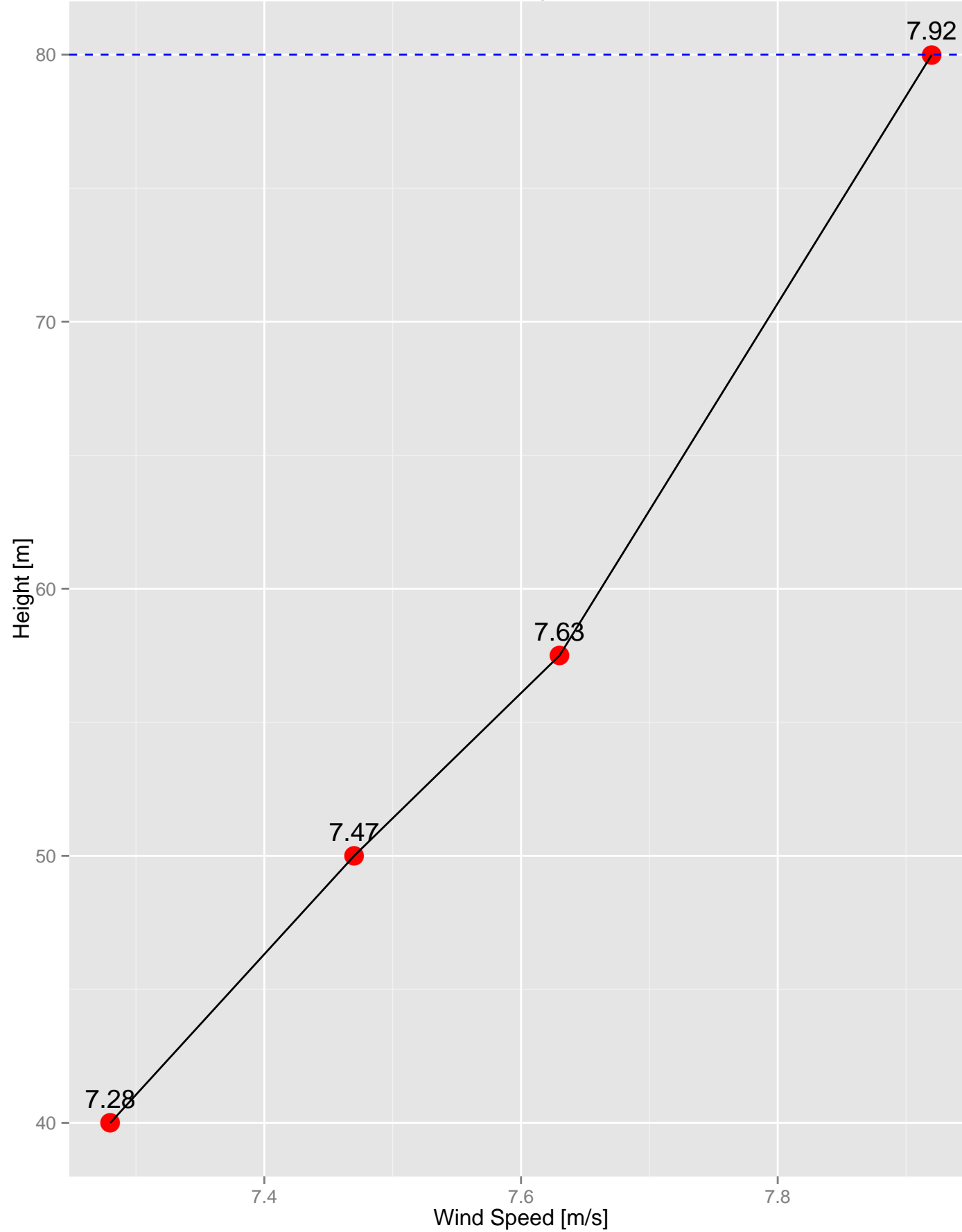
Shinagawa_8123_Hub Wind Speed Prediction, Data Period: 2019-11-12 14:40:00 – 2020-11-30 23:50:00 Number of Valid Data:54679, Hub Height:80m, Hub Wind Speed:7.92m/s
