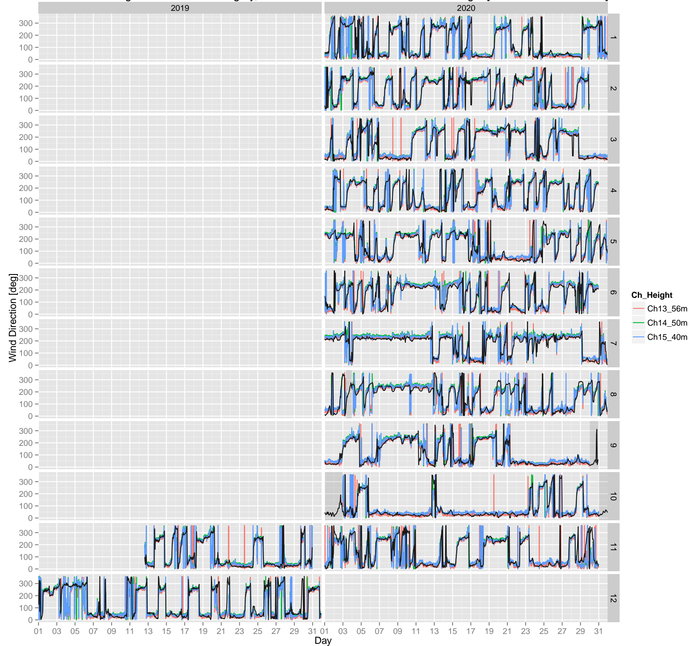
Akiruno_8342_Wind Direction_Time_Series (Data Period: 2019-11-12 14:40:00 – 2020-11-30 23:50:00) Periods of Missing data are shaded in grey, Black line is GPV-MSM data at 10m Height [Lat:34.8 Lon:139.0625]
