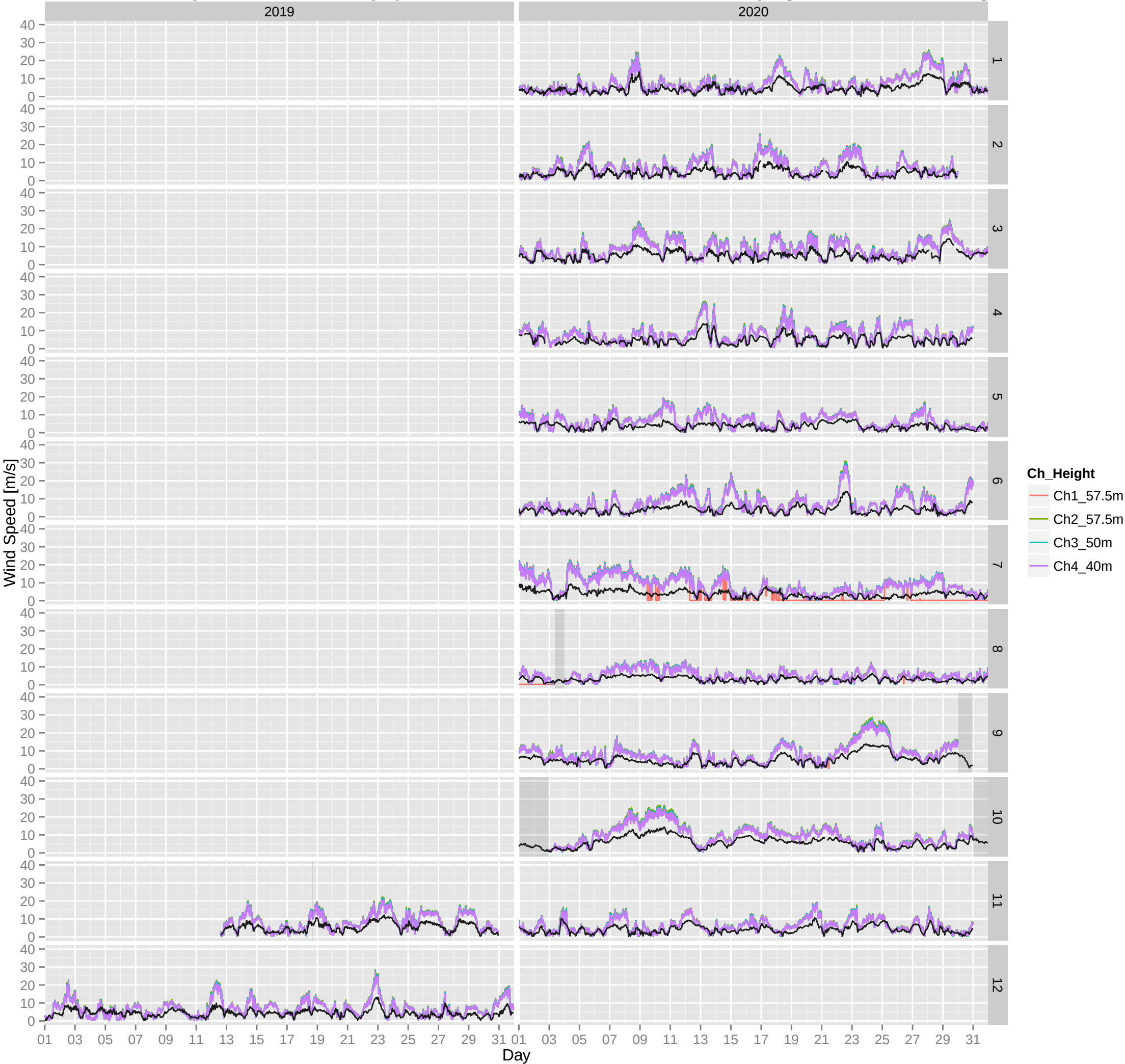
Akiruno_8342_Wind Speed_Time_Series (Data Period: 2019-11-12 14:40:00 – 2020-11-30 23:50:00) Periods of Missing data are shaded in grey, Black line is GPV-MSM data at 10m Height [Lat:34.8 Lon:139.0625]
